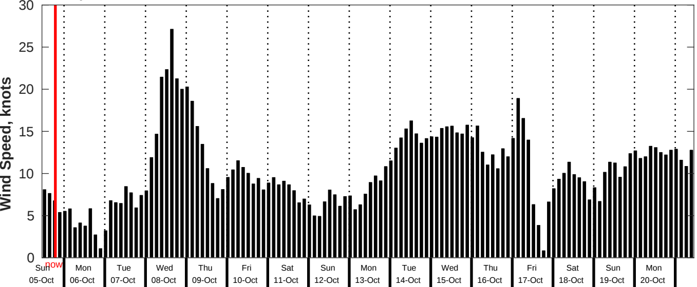
GFS Wind Speed Forecast for NDBC 52211 from 04-Oct-2025 11:00:00 to 20-Oct-2025 11:00:00
