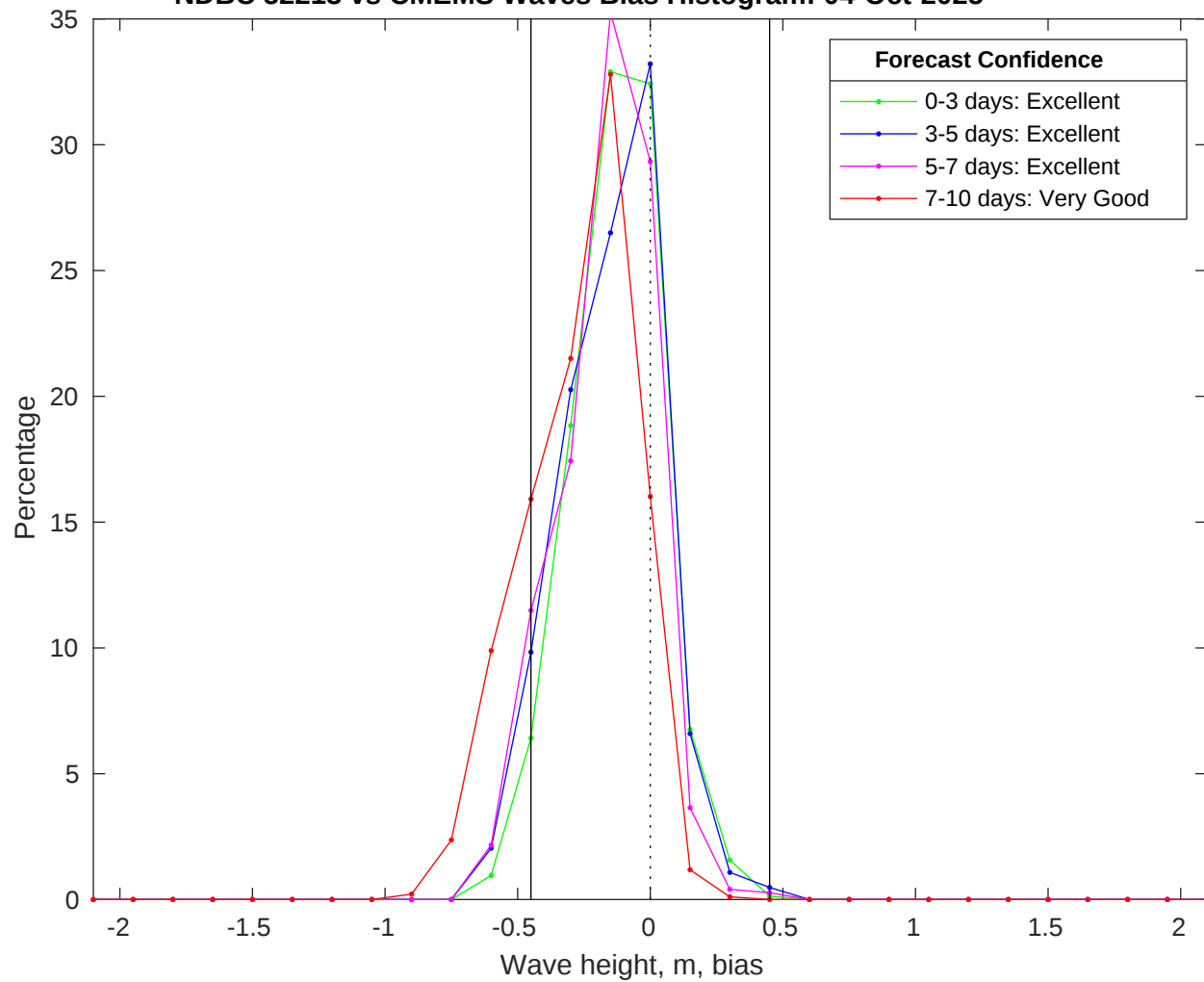
NDBC 52213 vs CMEMS Waves Bias Histogram: 04-Oct-2025
