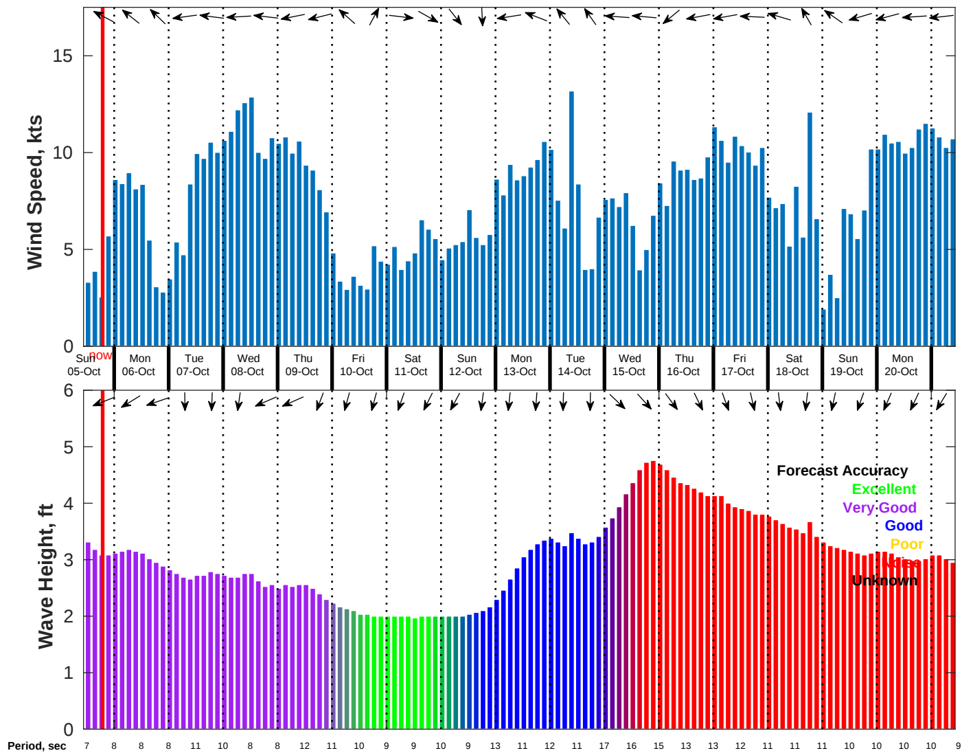
Wind & Wave Forecast for NDBC 52213 from 04-Oct-2025 11:00:00 to 20-Oct-2025 11:00:00
