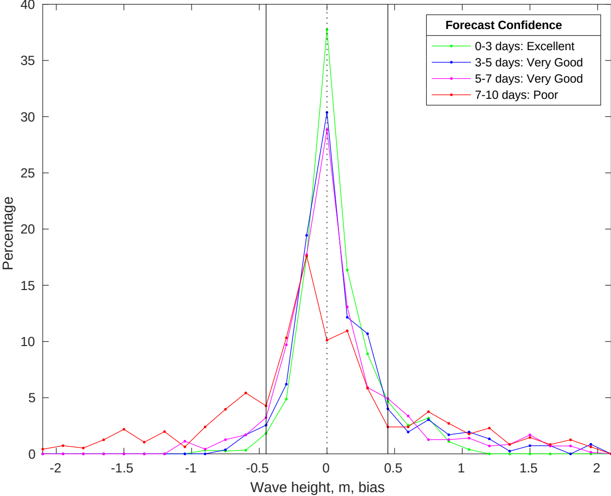
NDBC 41004 vs CMEMS Waves Bias Histogram: 05-Oct-2025
