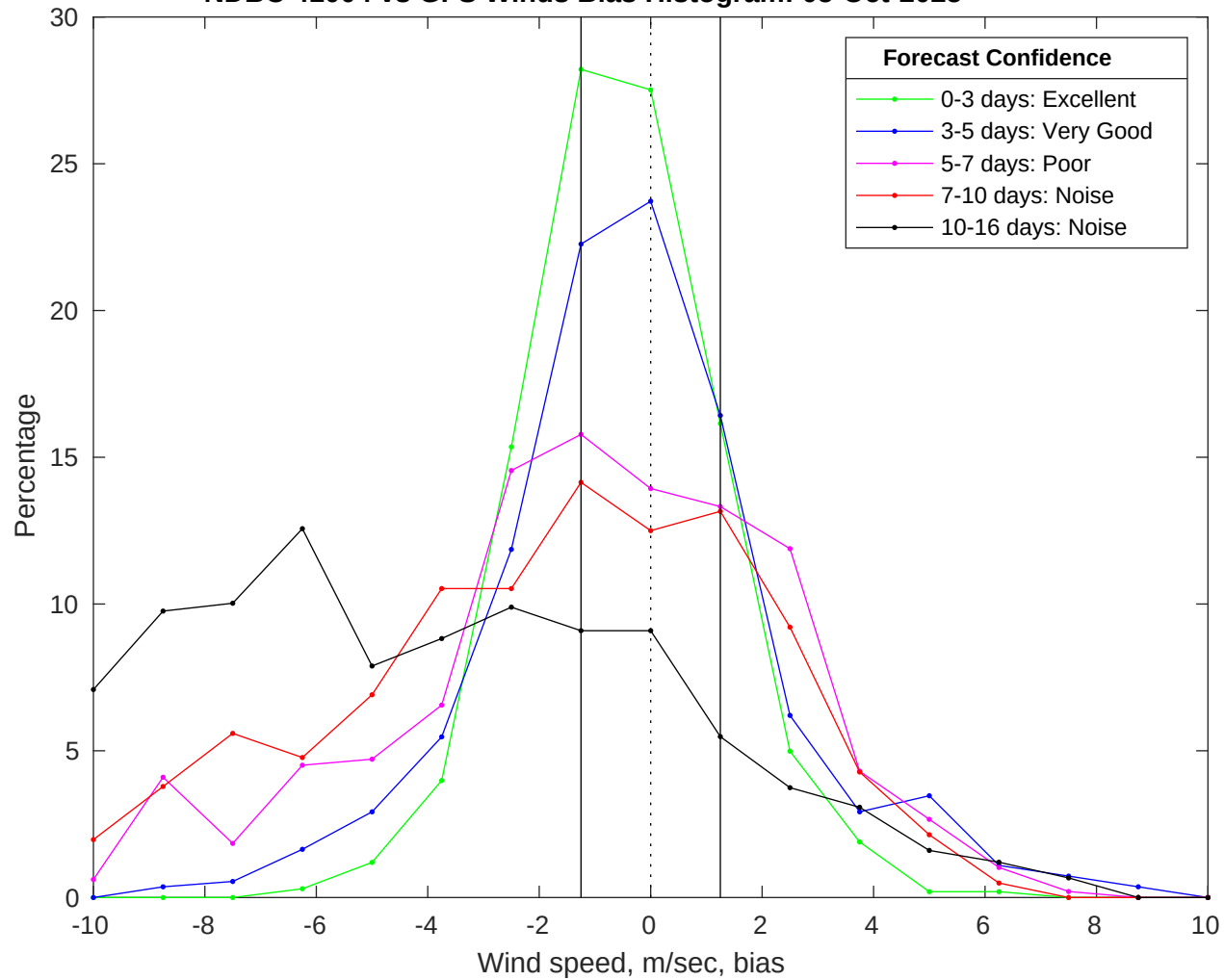
NDBC 41004 vs GFS Winds Bias Histogram: 05-Oct-2025
