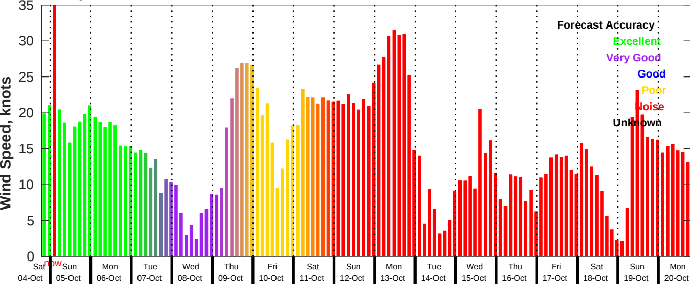
GFS Wind Speed Forecast for NDBC 41004 from 04-Oct-2025 19:00:00 to 20-Oct-2025 19:00:00
