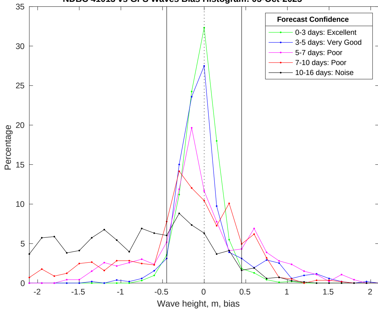
NDBC 41013 vs GFS Waves Bias Histogram: 05-Oct-2025
