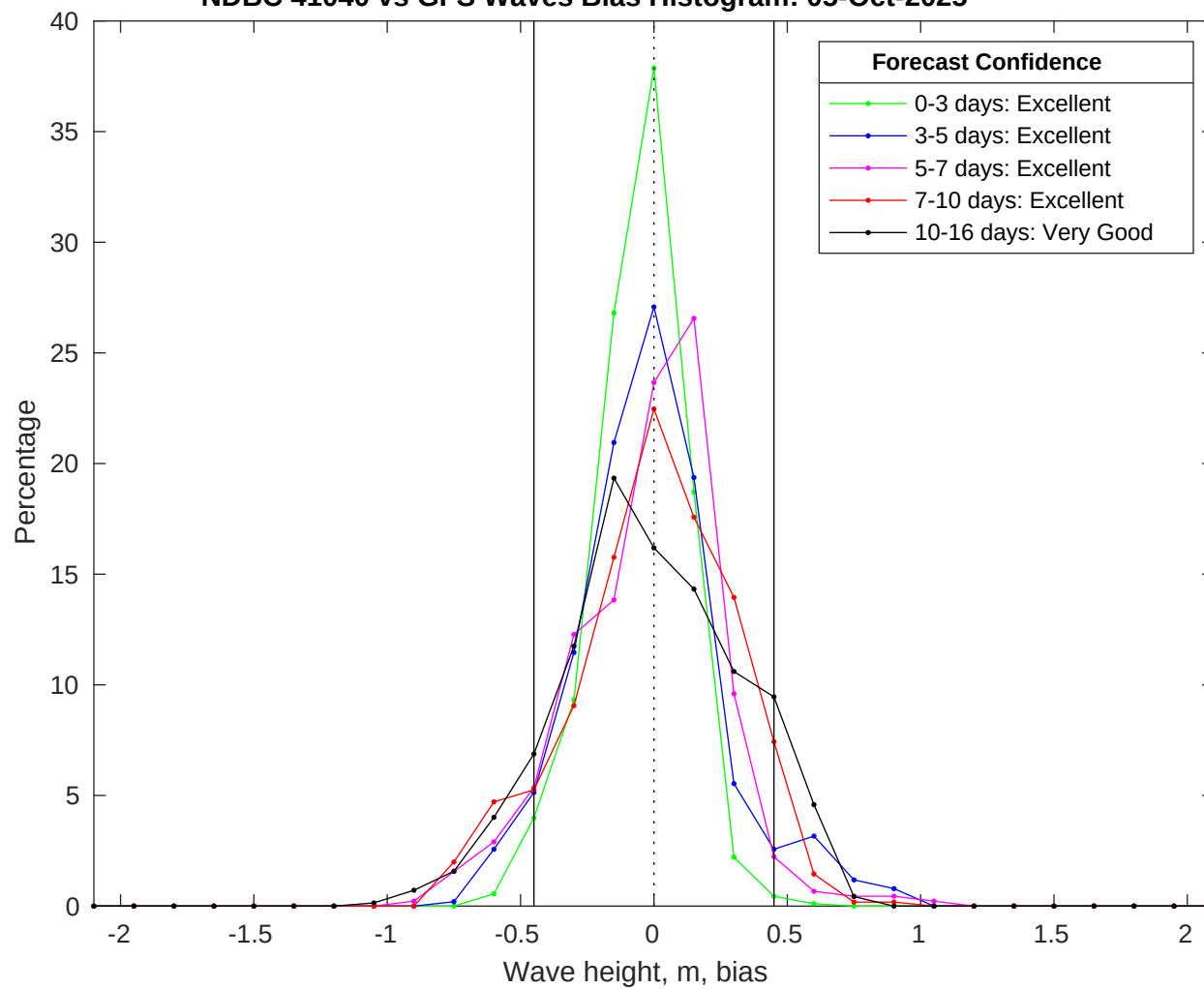
NDBC 41040 vs GFS Waves Bias Histogram: 05-Oct-2025
