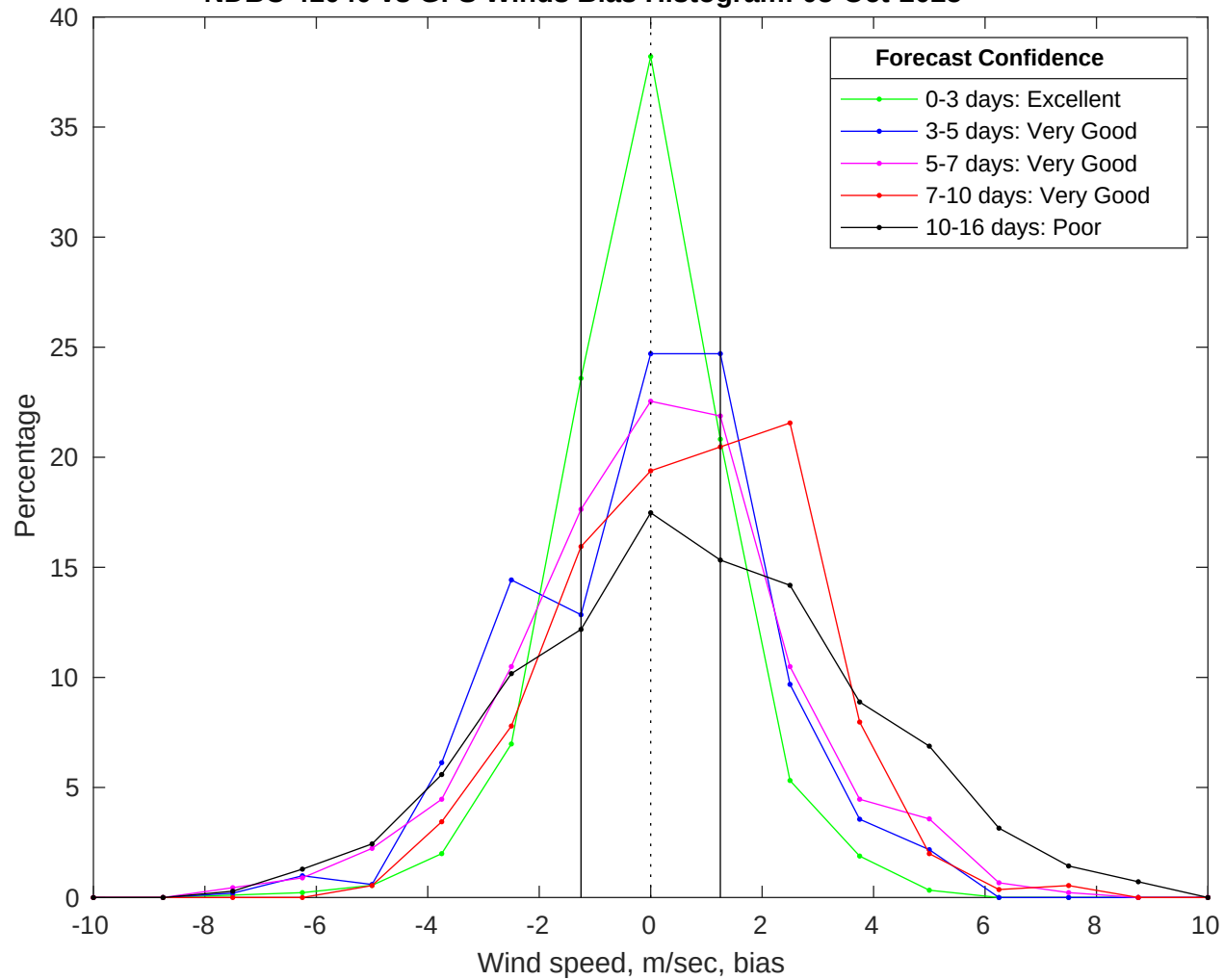
NDBC 41040 vs GFS Winds Bias Histogram: 05-Oct-2025
