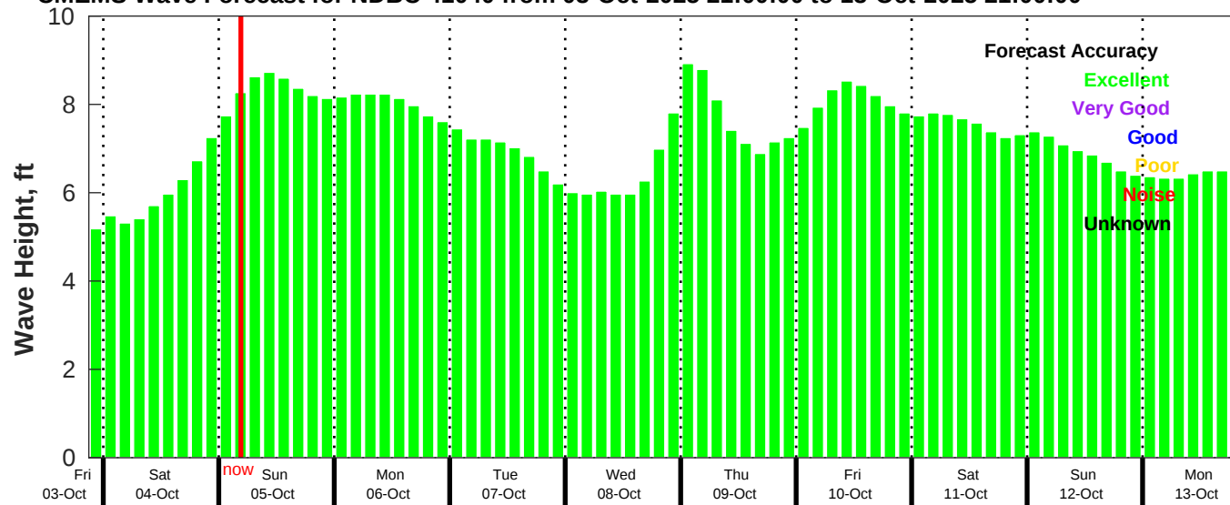
CMEMS Wave Forecast for NDBC 41040 from 03-Oct-2025 21:00:00 to 13-Oct-2025 21:00:00
