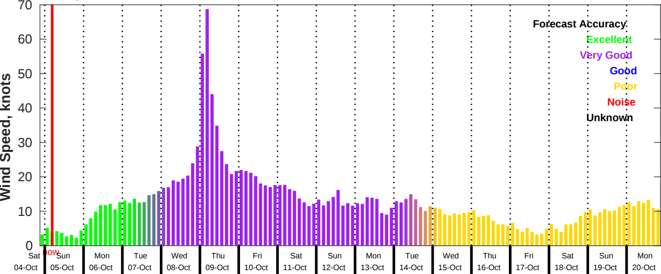
GFS Wind Speed Forecast for NDBC 41040 from 04-Oct-2025 21:00:00 to 20-Oct-2025 21:00:00
