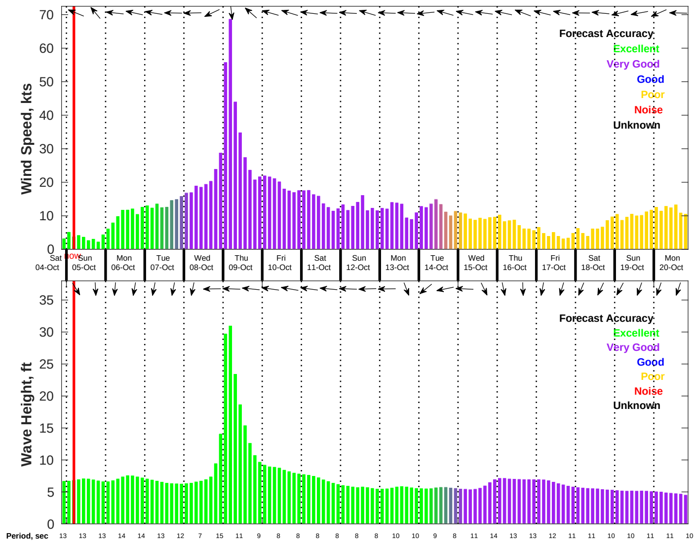
Wind & Wave Forecast for NDBC 41040 from 04-Oct-2025 21:00:00 to 20-Oct-2025 21:00:00
