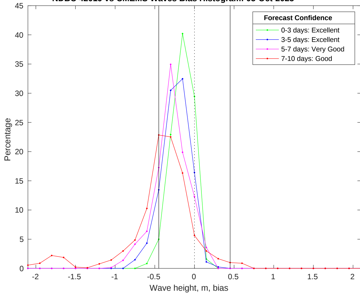
NDBC 42019 vs CMEMS Waves Bias Histogram: 05-Oct-2025
