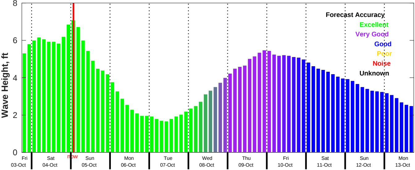
CMEMS Wave Forecast for NDBC 42019 from 03-Oct-2025 18:00:00 to 13-Oct-2025 18:00:00
