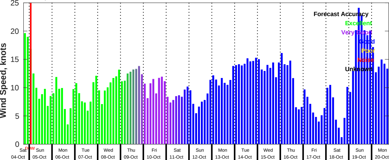
GFS Wind Speed Forecast for NDBC 42019 from 04-Oct-2025 18:00:00 to 20-Oct-2025 18:00:00
