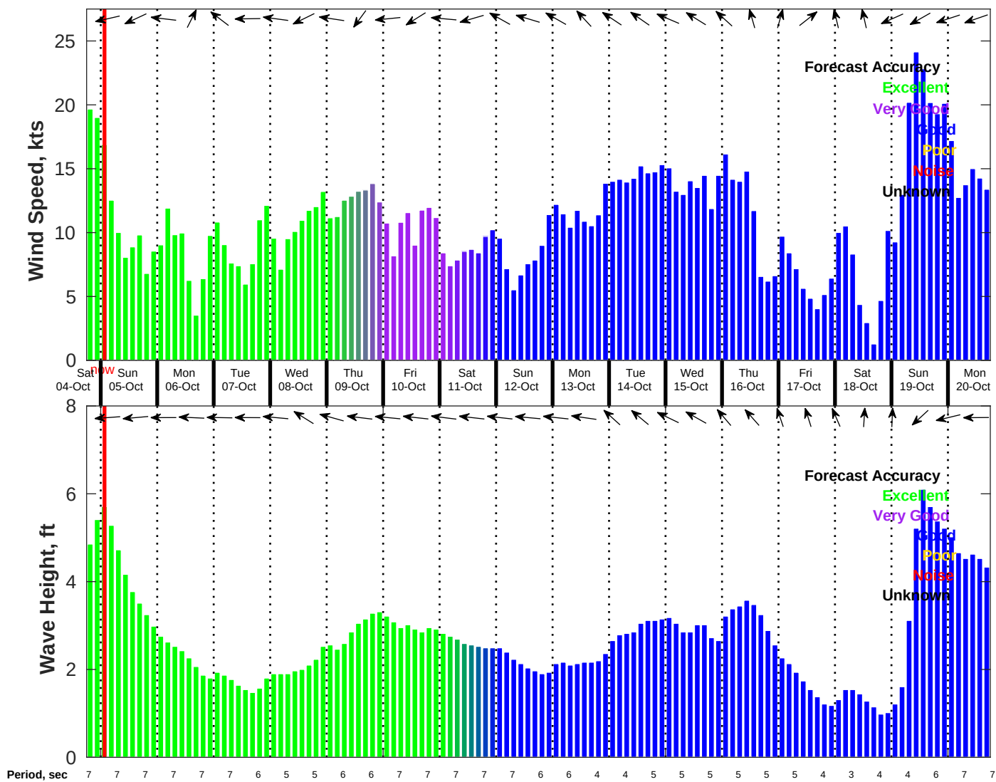
Wind & Wave Forecast for NDBC 42019 from 04-Oct-2025 18:00:00 to 20-Oct-2025 18:00:00
