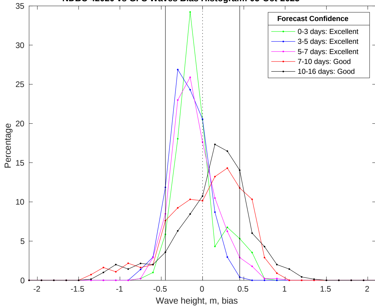
NDBC 42020 vs GFS Waves Bias Histogram: 05-Oct-2025
