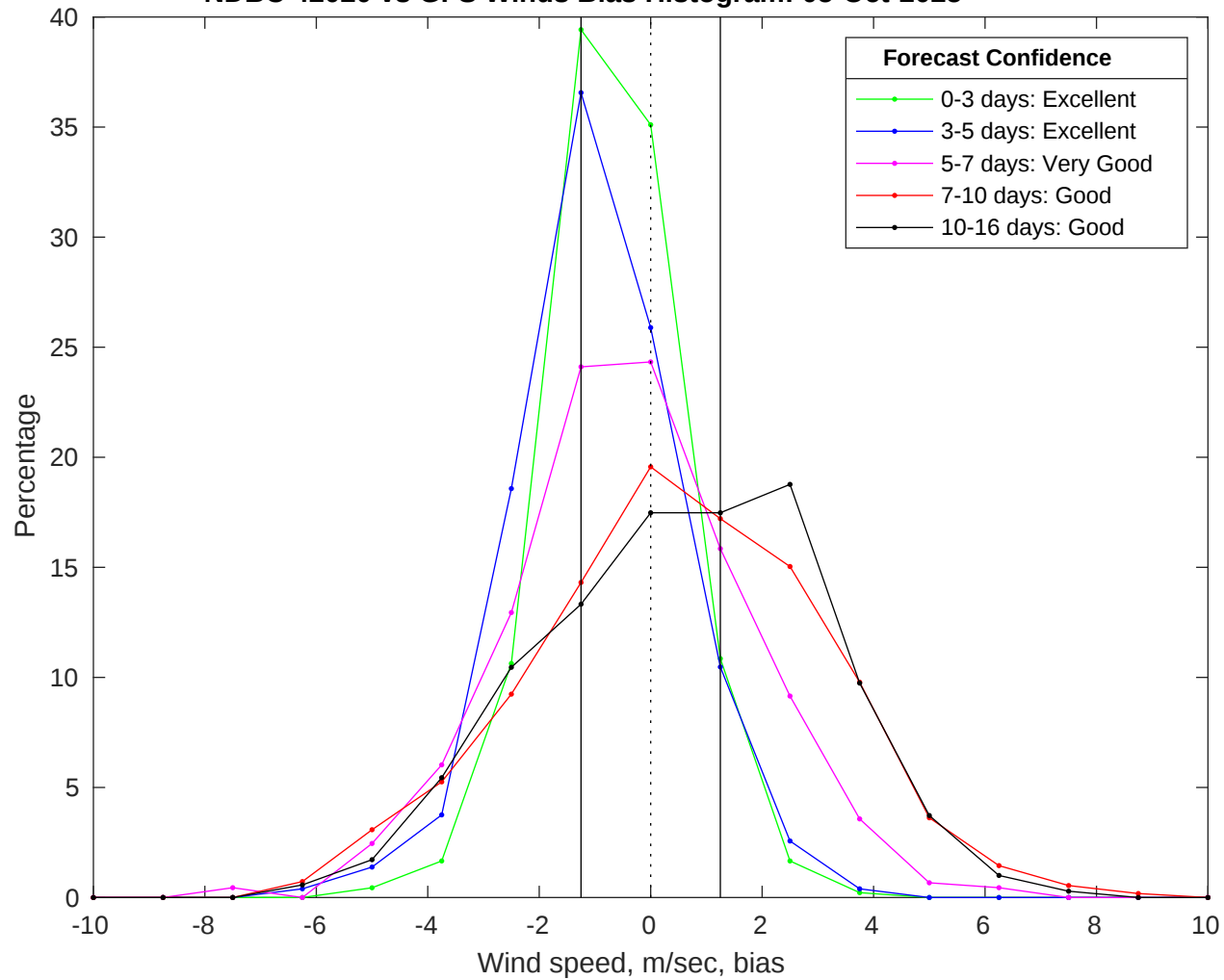
NDBC 42020 vs GFS Winds Bias Histogram: 05-Oct-2025
