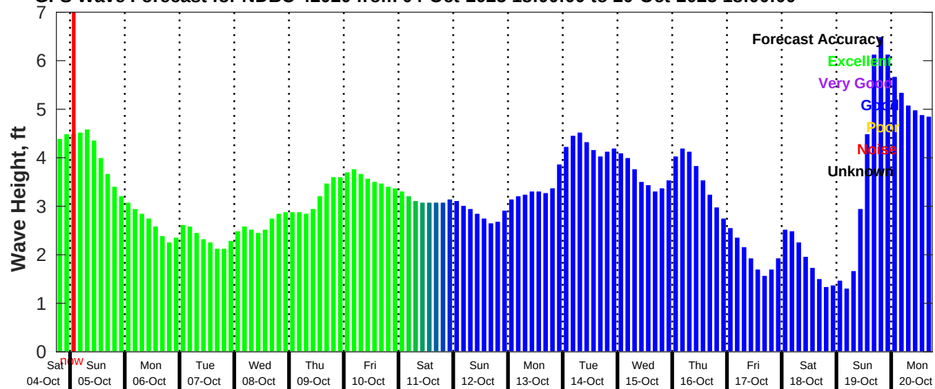
GFS Wave Forecast for NDBC 42020 from 04-Oct-2025 18:00:00 to 20-Oct-2025 18:00:00
