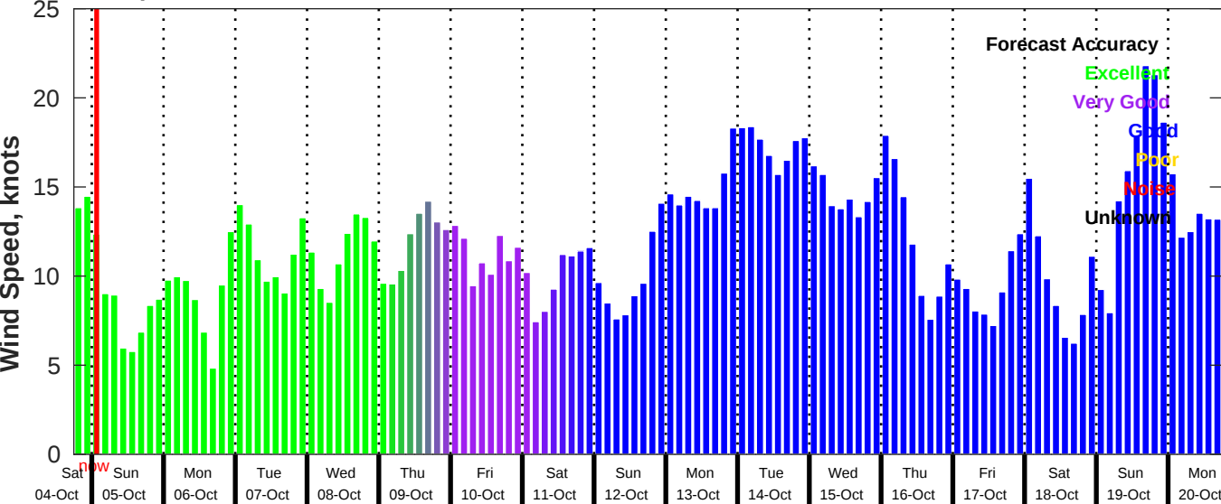
GFS Wind Speed Forecast for NDBC 42020 from 04-Oct-2025 18:00:00 to 20-Oct-2025 18:00:00
