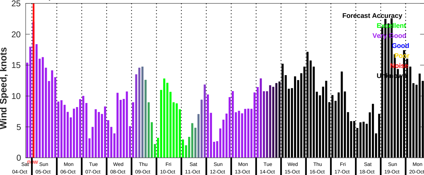
GFS Wind Speed Forecast for NDBC 42035 from 04-Oct-2025 18:00:00 to 20-Oct-2025 18:00:00
