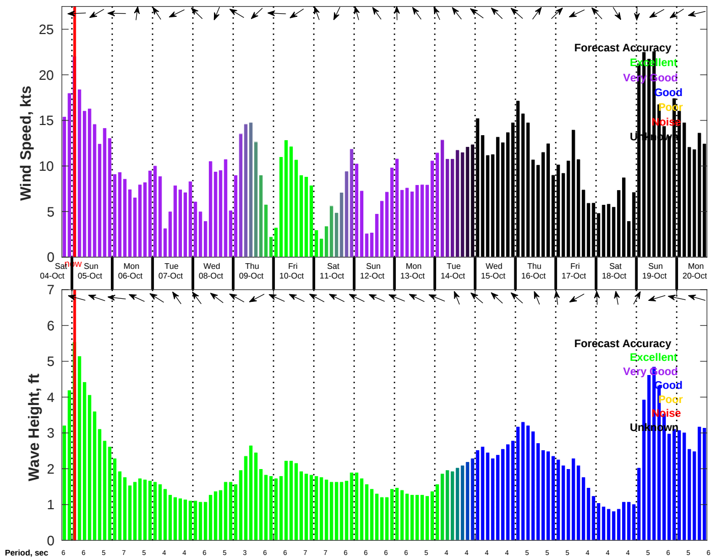
Wind & Wave Forecast for NDBC 42035 from 04-Oct-2025 18:00:00 to 20-Oct-2025 18:00:00
