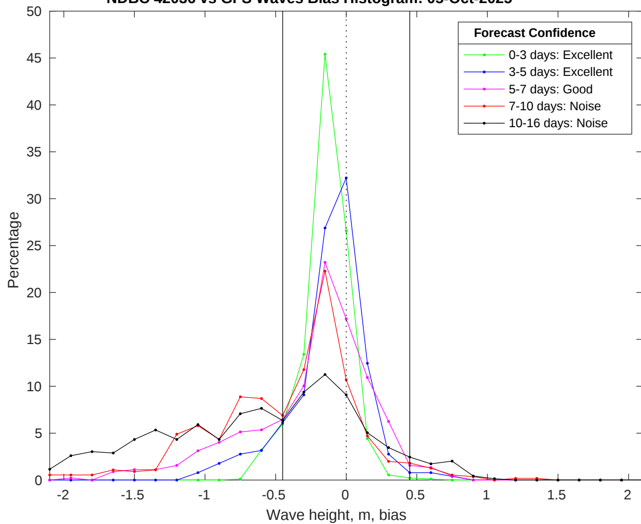
NDBC 42036 vs GFS Waves Bias Histogram: 05-Oct-2025
