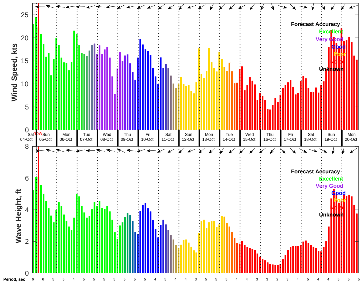
Wind & Wave Forecast for NDBC 42036 from 04-Oct-2025 19:00:00 to 20-Oct-2025 19:00:00
