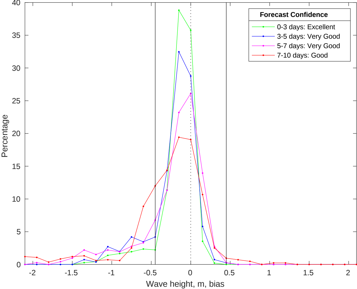
NDBC 42040 vs CMEMS Waves Bias Histogram: 05-Oct-2025
