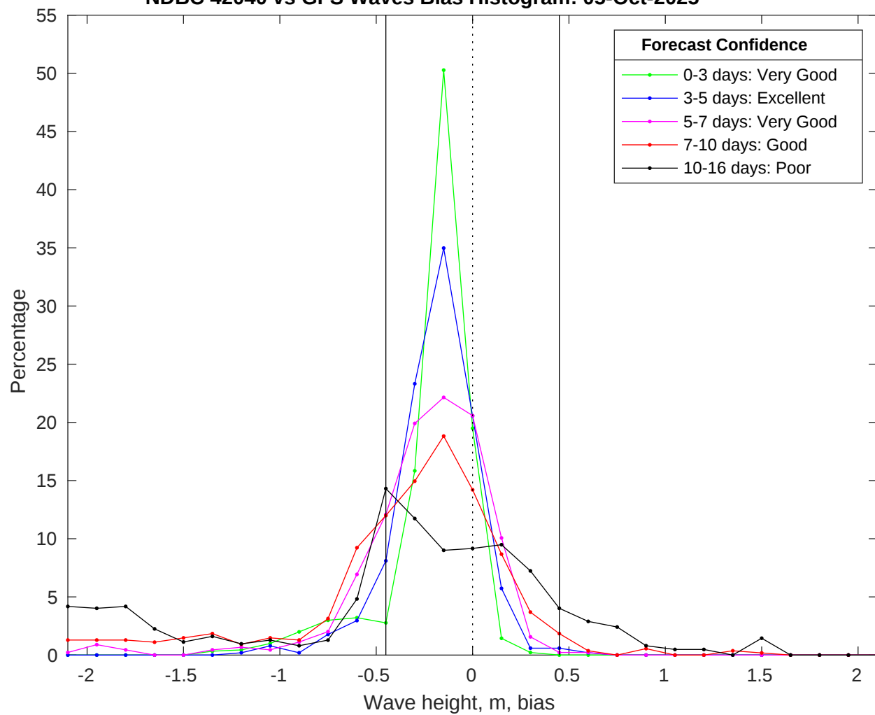
NDBC 42040 vs GFS Waves Bias Histogram: 05-Oct-2025
