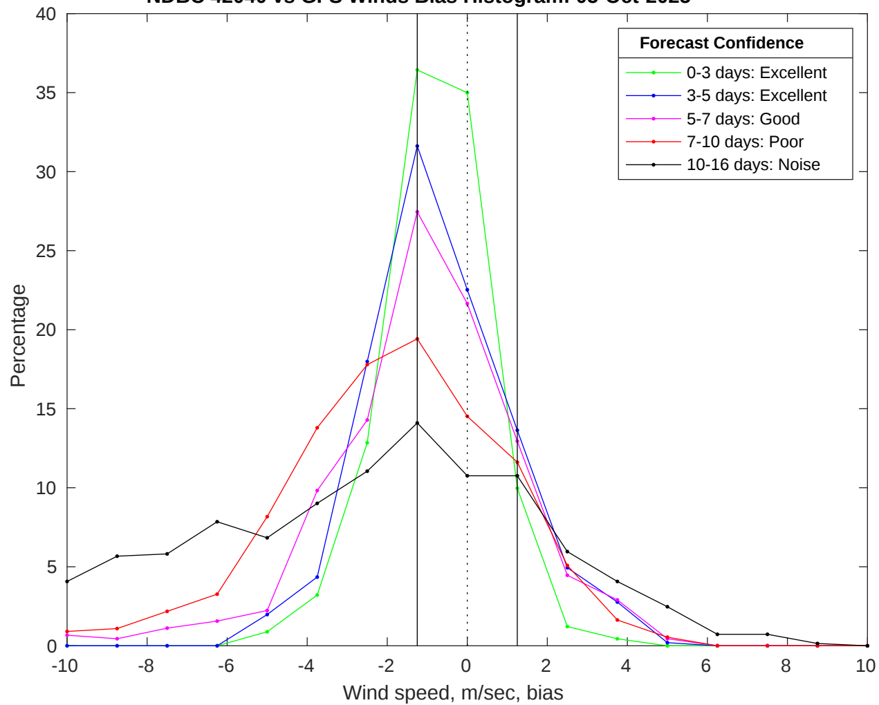
NDBC 42040 vs GFS Winds Bias Histogram: 05-Oct-2025
