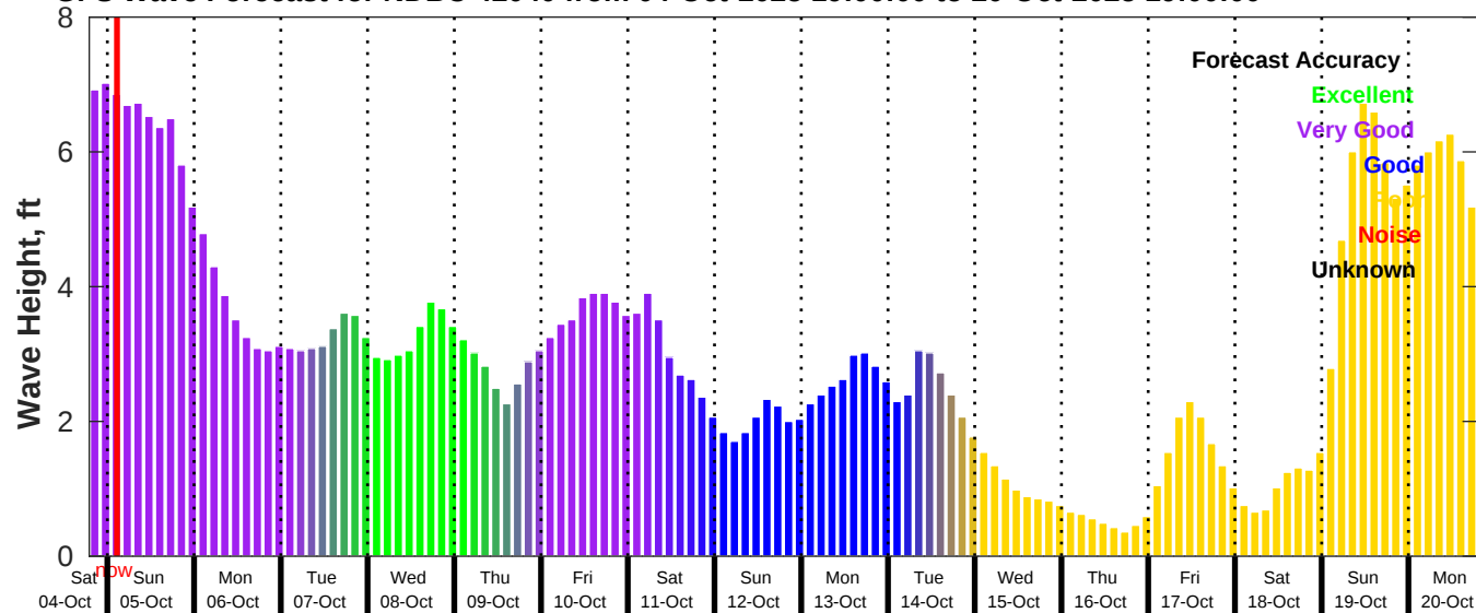
GFS Wave Forecast for NDBC 42040 from 04-Oct-2025 19:00:00 to 20-Oct-2025 19:00:00
