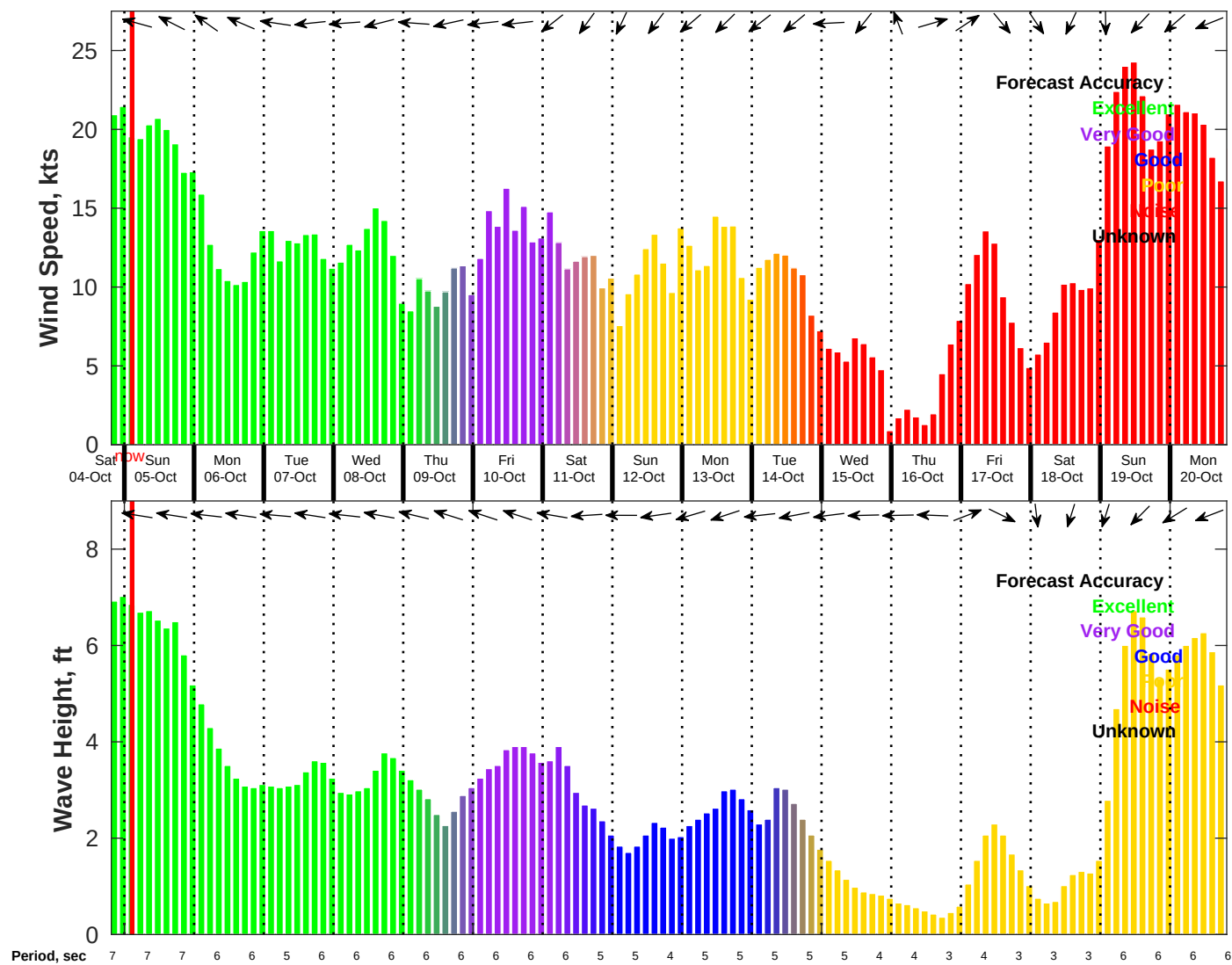
Wind & Wave Forecast for NDBC 42040 from 04-Oct-2025 19:00:00 to 20-Oct-2025 19:00:00
