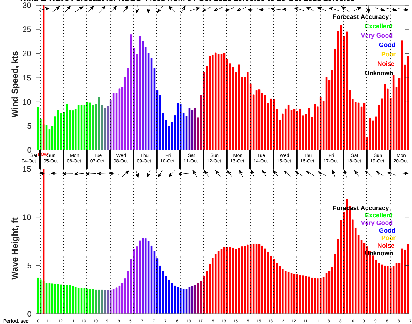
Wind & Wave Forecast for NDBC 44008 from 04-Oct-2025 20:00:00 to 20-Oct-2025 20:00:00
