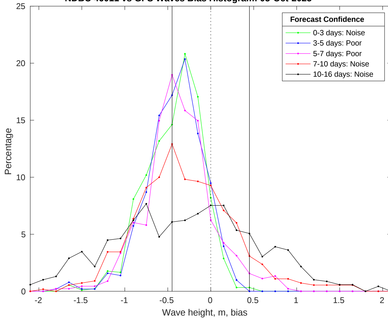
NDBC 46011 vs GFS Waves Bias Histogram: 05-Oct-2025
