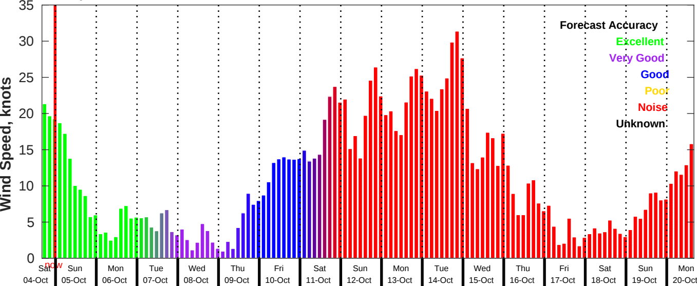
GFS Wind Speed Forecast for NDBC 46011 from 04-Oct-2025 16:00:00 to 20-Oct-2025 16:00:00
