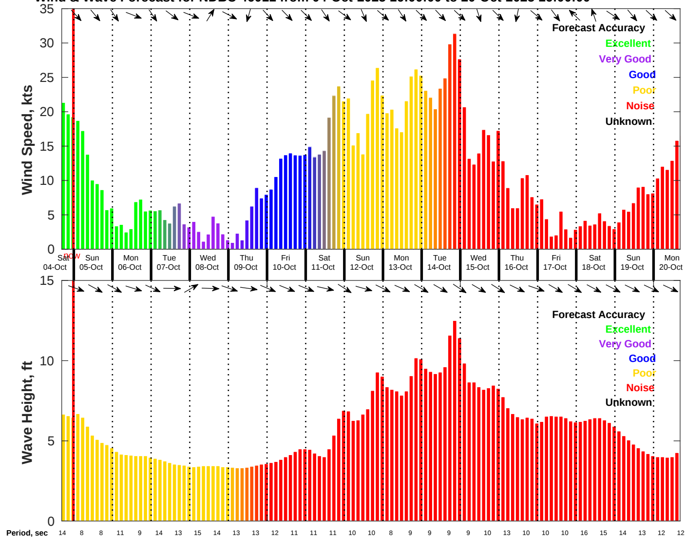
Wind & Wave Forecast for NDBC 46011 from 04-Oct-2025 16:00:00 to 20-Oct-2025 16:00:00
