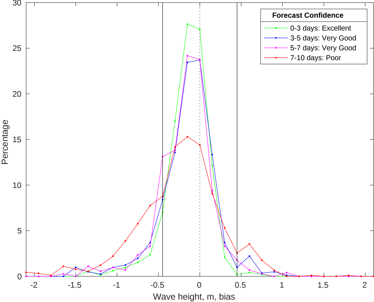
NDBC 46028 vs CMEMS Waves Bias Histogram: 05-Oct-2025
