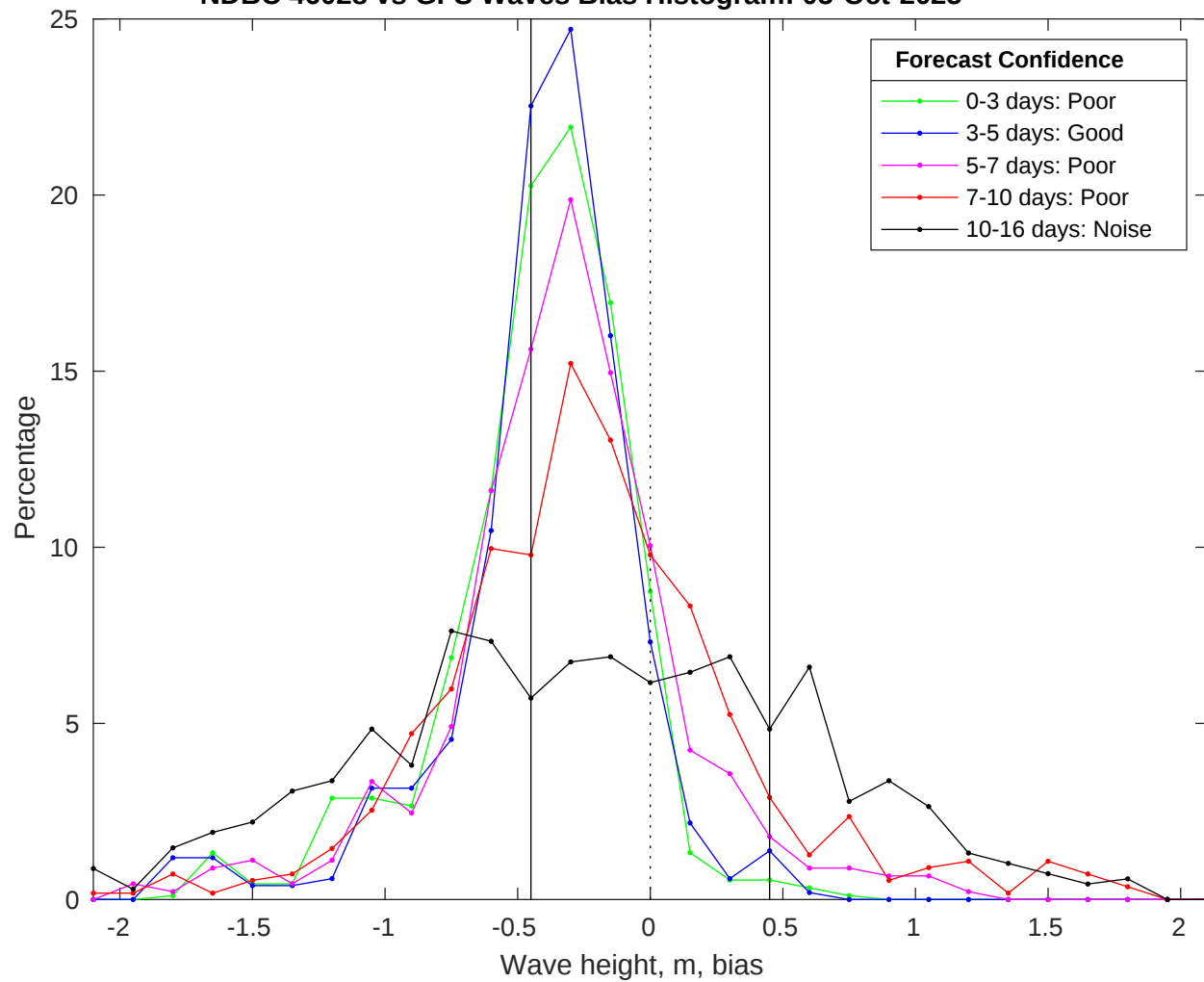
NDBC 46028 vs GFS Waves Bias Histogram: 05-Oct-2025
