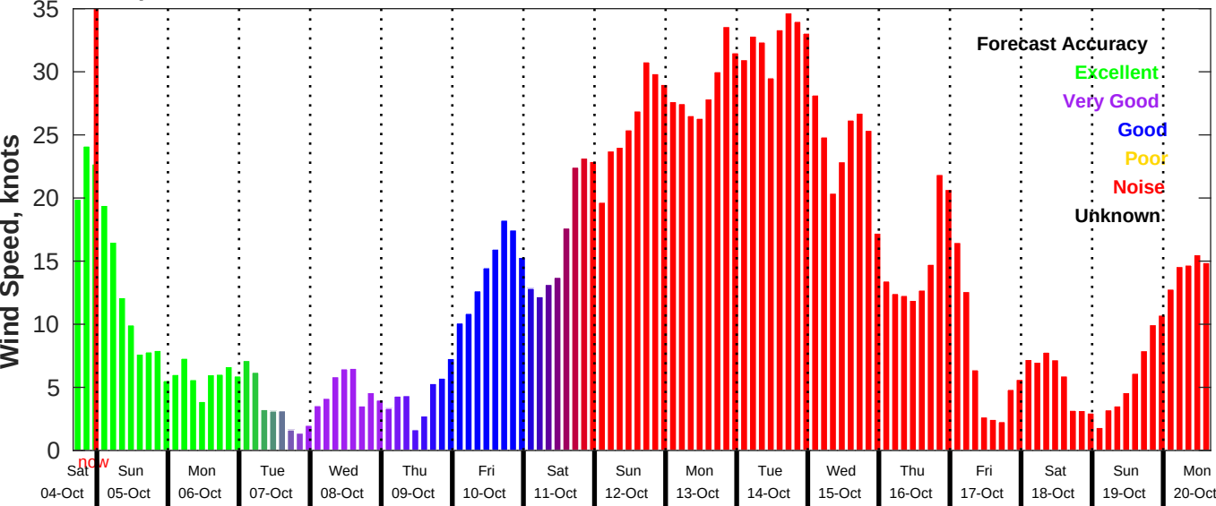
GFS Wind Speed Forecast for NDBC 46028 from 04-Oct-2025 16:00:00 to 20-Oct-2025 16:00:00
