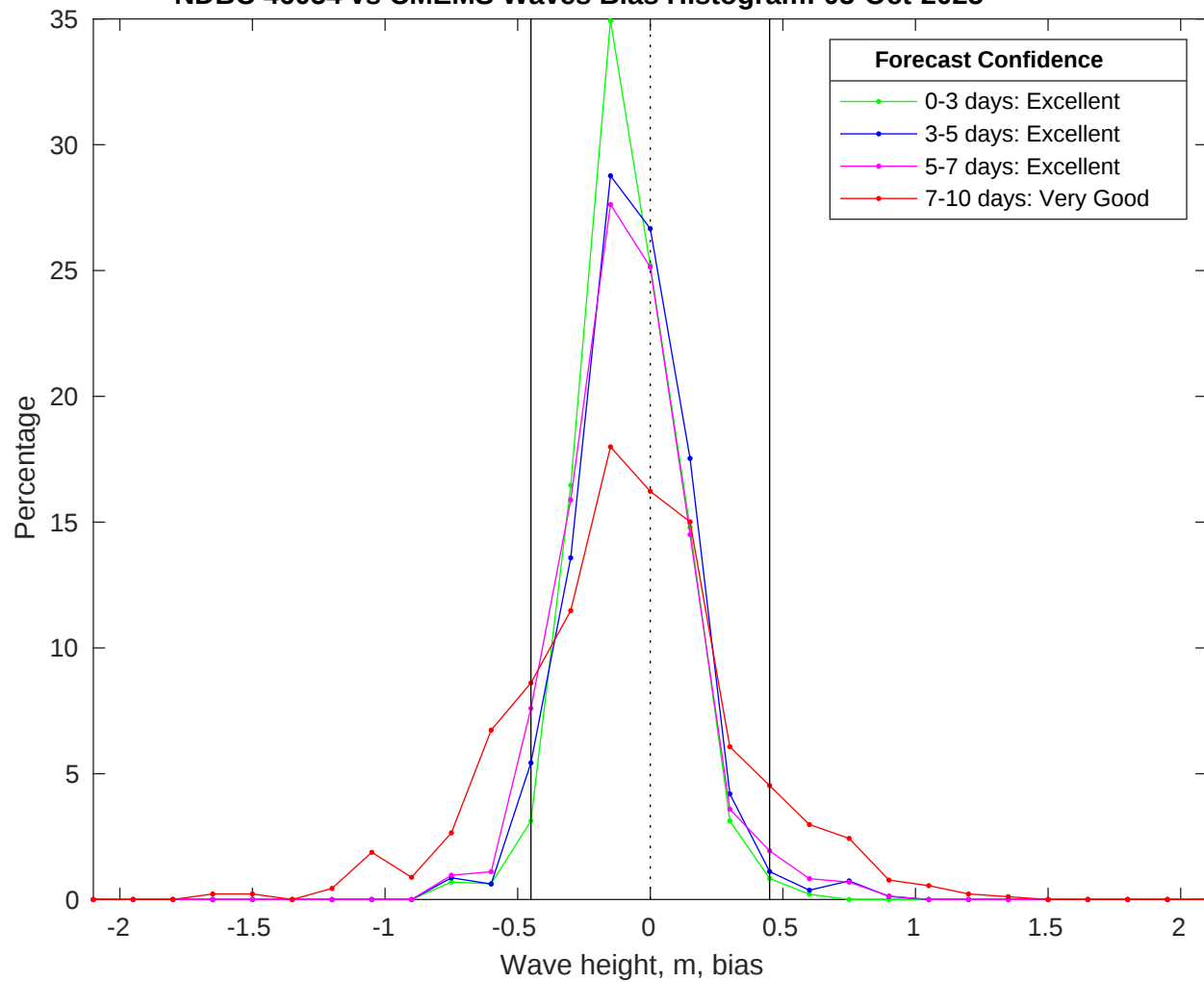
NDBC 46054 vs CMEMS Waves Bias Histogram: 05-Oct-2025
