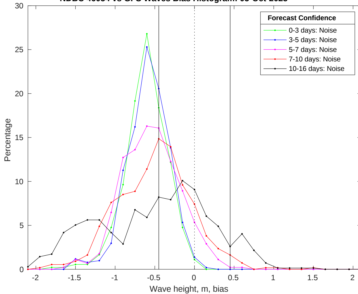
NDBC 46054 vs GFS Waves Bias Histogram: 05-Oct-2025
