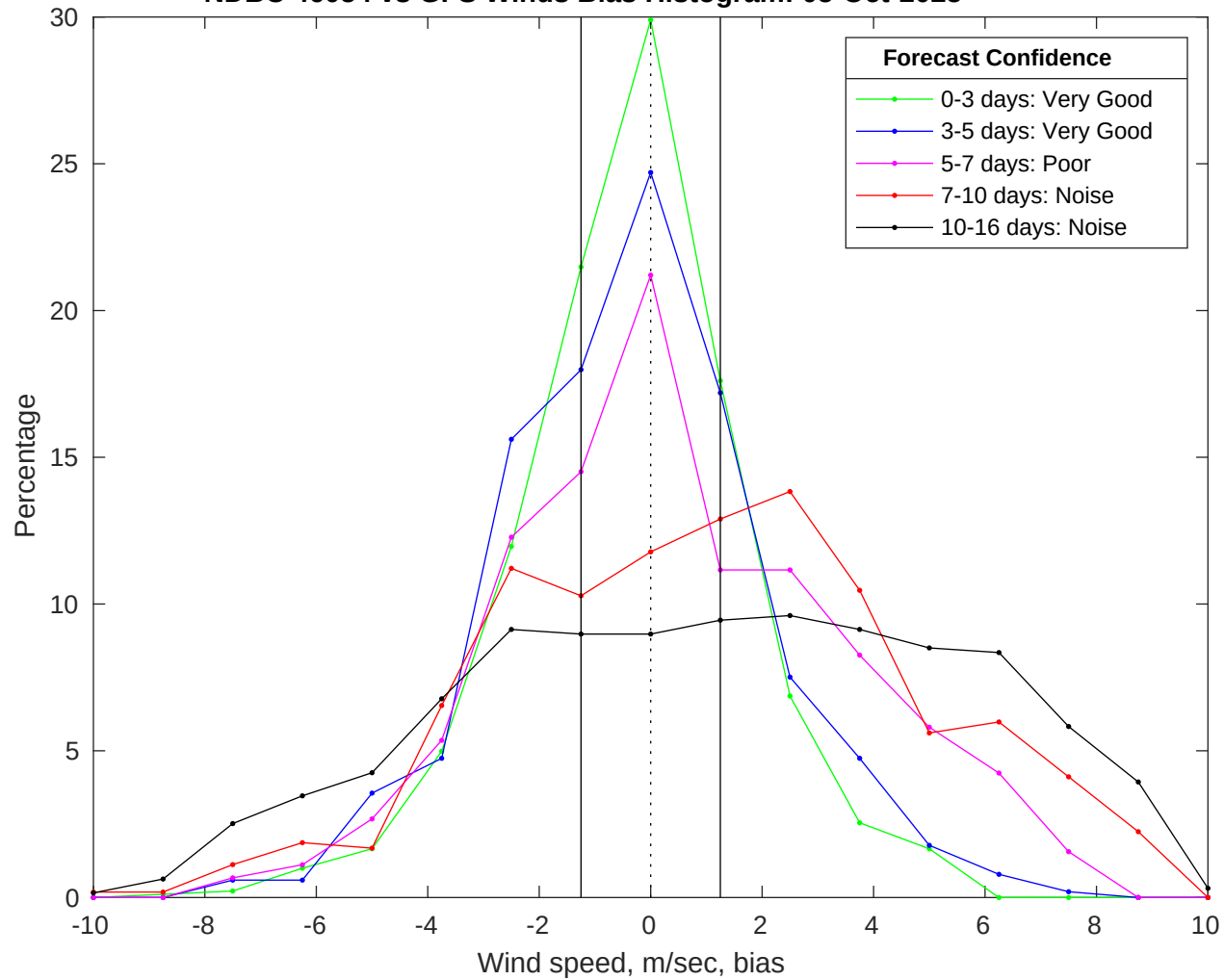
NDBC 46054 vs GFS Winds Bias Histogram: 05-Oct-2025
