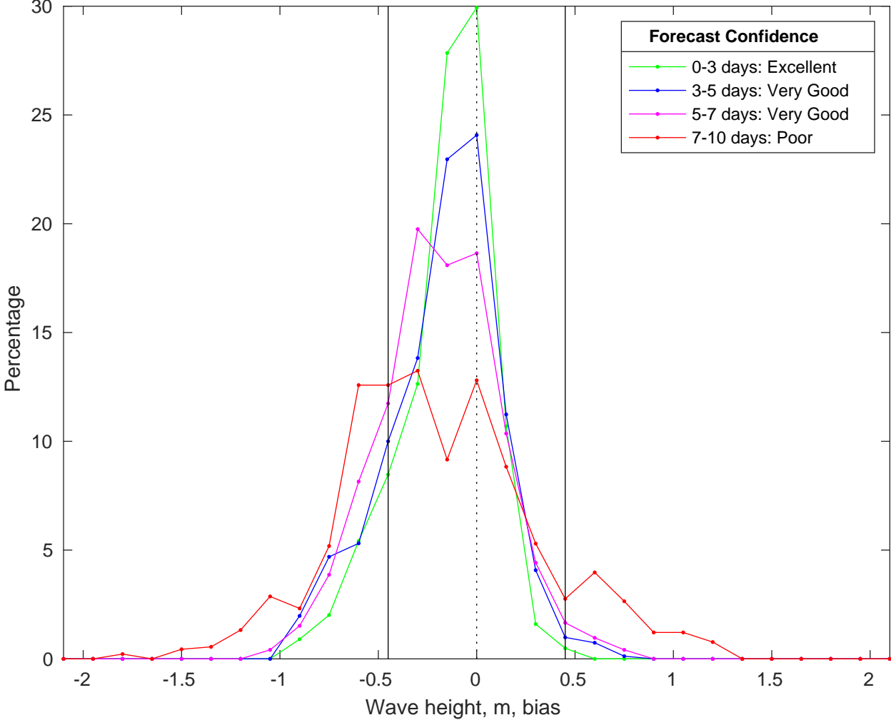
NDBC 46069 vs CMEMS Waves Bias Histogram: 05-Oct-2025
