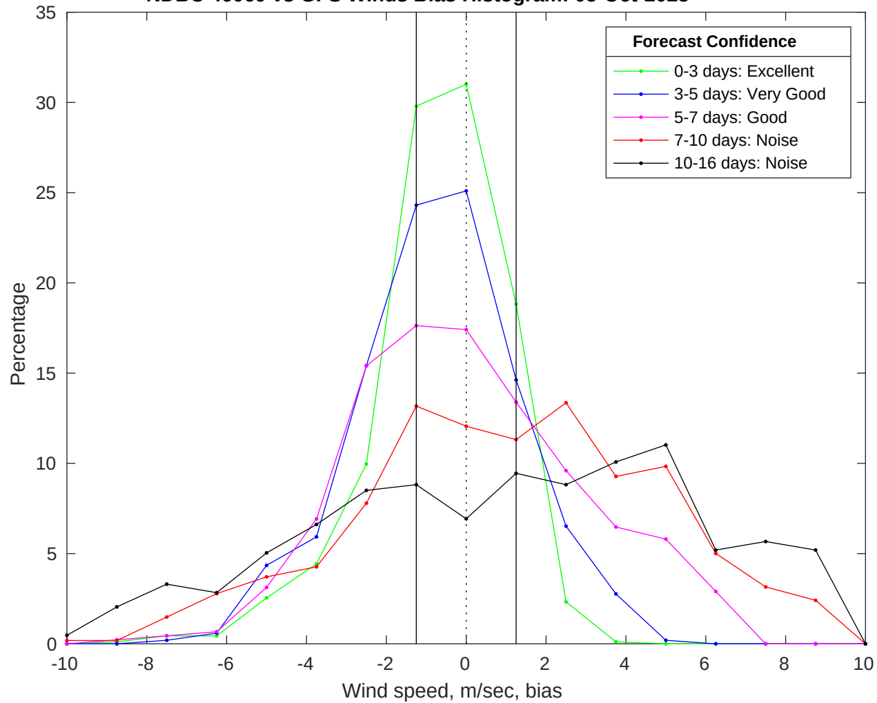
NDBC 46069 vs GFS Winds Bias Histogram: 05-Oct-2025
