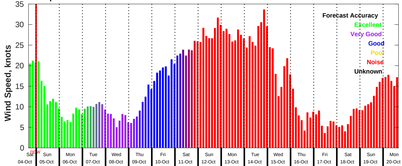
GFS Wind Speed Forecast for NDBC 46069 from 04-Oct-2025 16:00:00 to 20-Oct-2025 16:00:00
