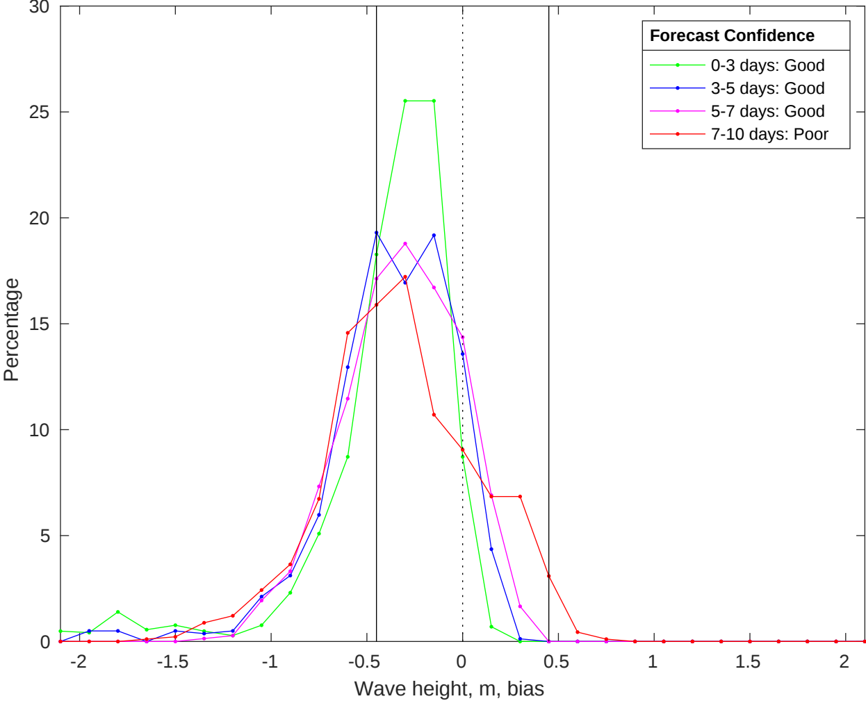
NDBC 51209 vs CMEMS Waves Bias Histogram: 05-Oct-2025
