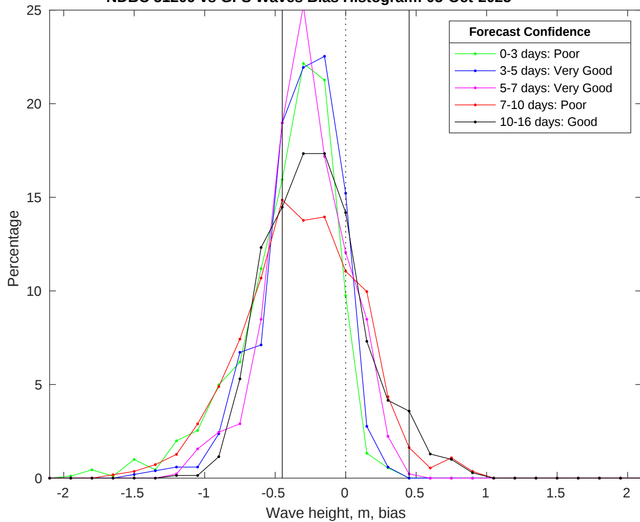
NDBC 51209 vs GFS Waves Bias Histogram: 05-Oct-2025
