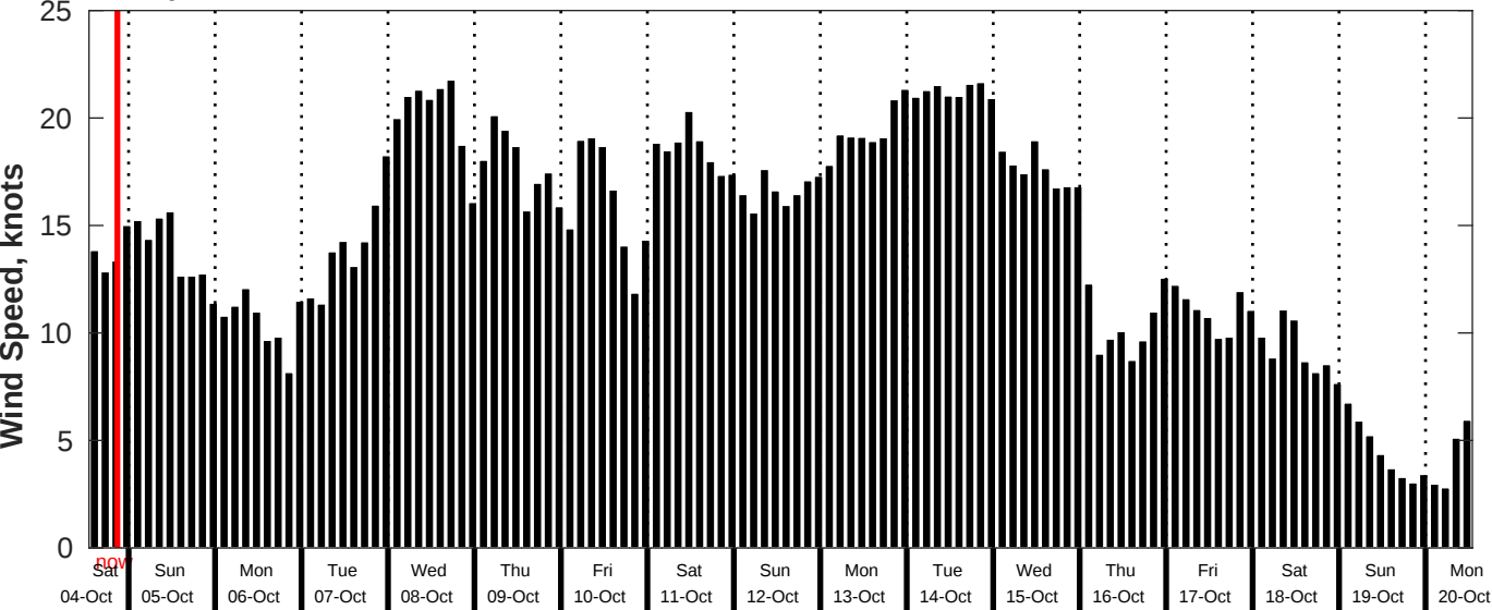
GFS Wind Speed Forecast for NDBC 51209 from 04-Oct-2025 13:00:00 to 20-Oct-2025 13:00:00
