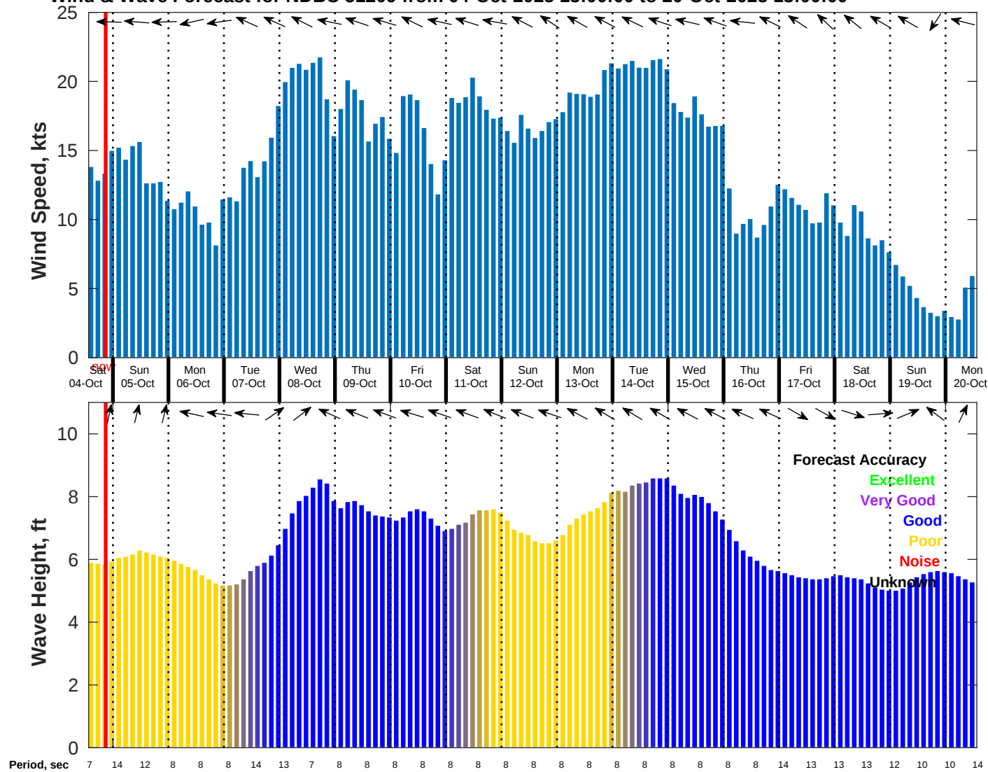
Wind & Wave Forecast for NDBC 51209 from 04-Oct-2025 13:00:00 to 20-Oct-2025 13:00:00
