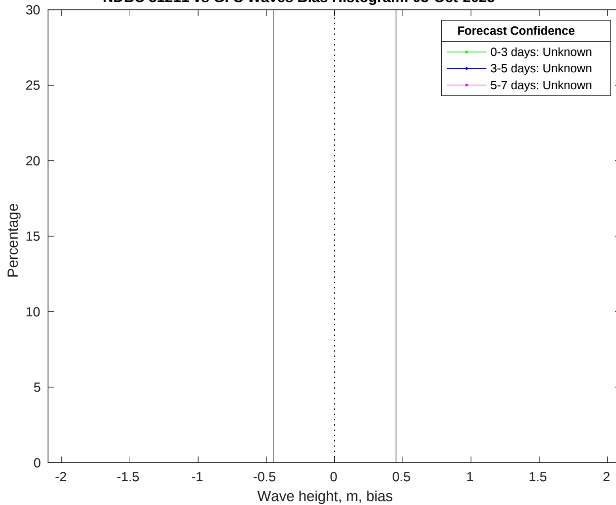
NDBC 51211 vs GFS Waves Bias Histogram: 05-Oct-2025
