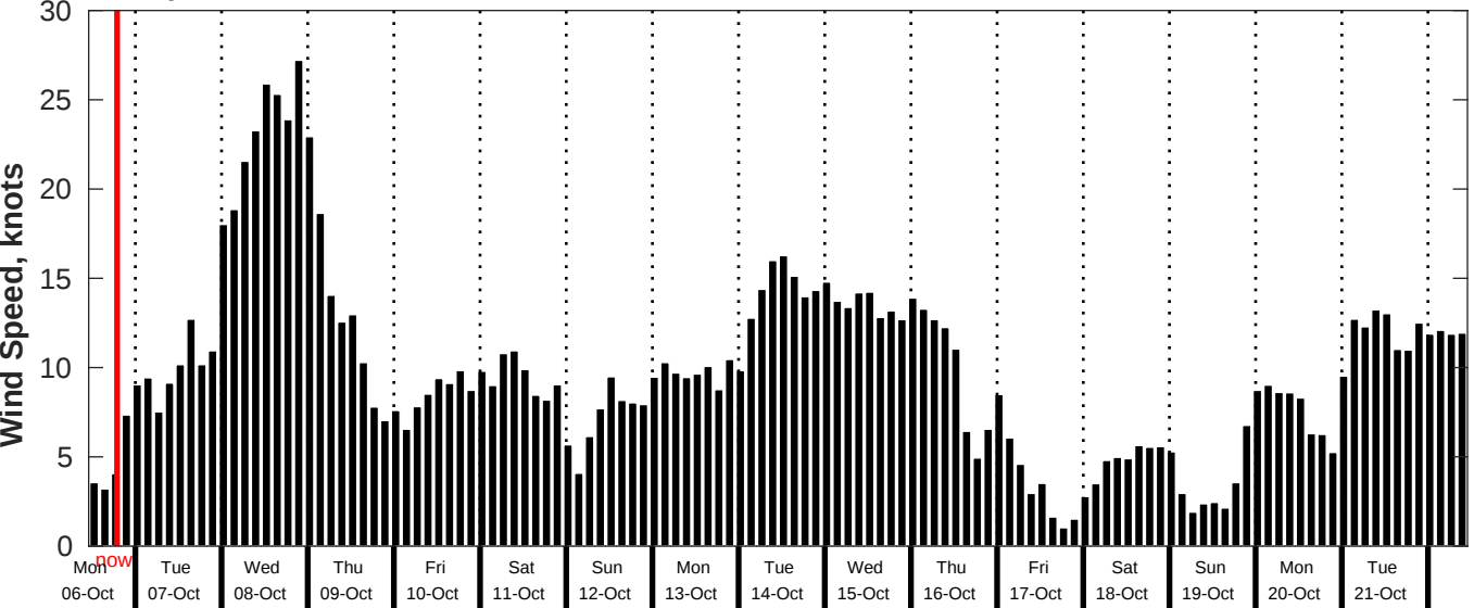
GFS Wind Speed Forecast for NDBC 52211 from 05-Oct-2025 11:00:00 to 21-Oct-2025 11:00:00
