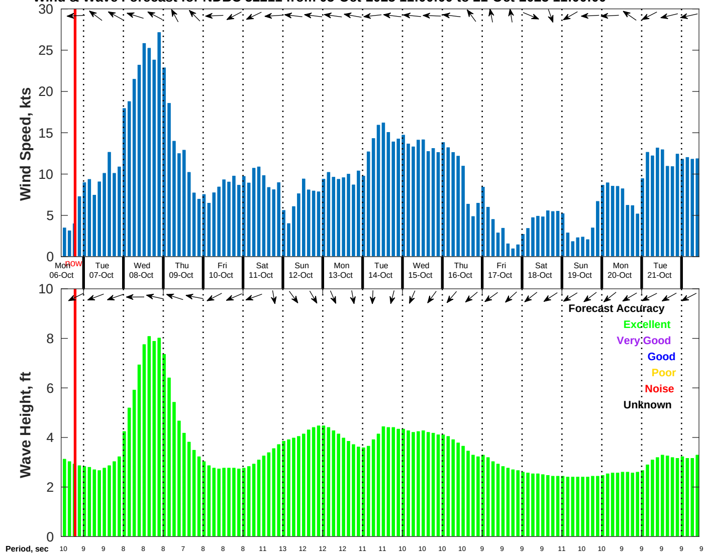
Wind & Wave Forecast for NDBC 52211 from 05-Oct-2025 11:00:00 to 21-Oct-2025 11:00:00
