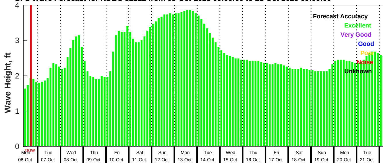
GFS Wave Forecast for NDBC 52212 from 05-Oct-2025 09:00:00 to 21-Oct-2025 09:00:00
